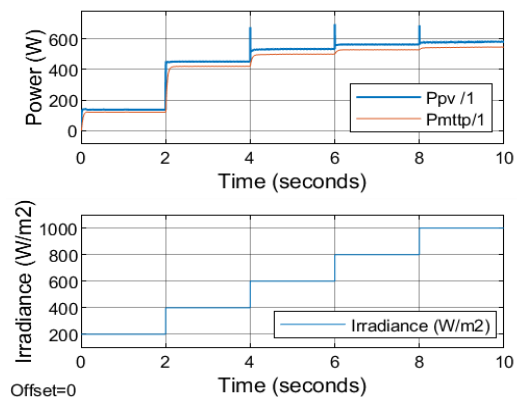
Fig. 6. PV array and MPPT output power.
