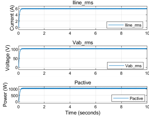
Fig. 8. RMS voltage, current and active power ( P_{active} ) at the rated wind speed of 10m/s.
