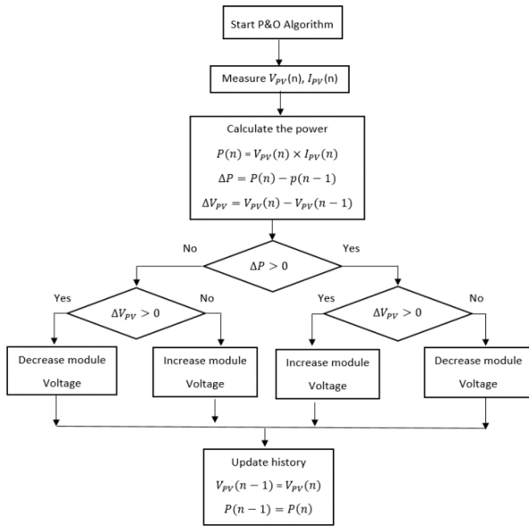
Fig. 4. P&amp;O algorithm flow chart [18].
