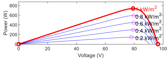
Fig. 7. Array P-V characteristic curve for different irradiance levels.
