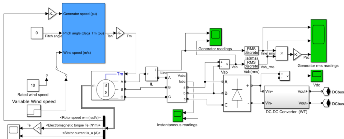
Fig. 3. Wind turbine model in Simulink with PMSG and Rectifier.
