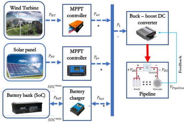
Fig. 1. Proposed system schematic diagram.
