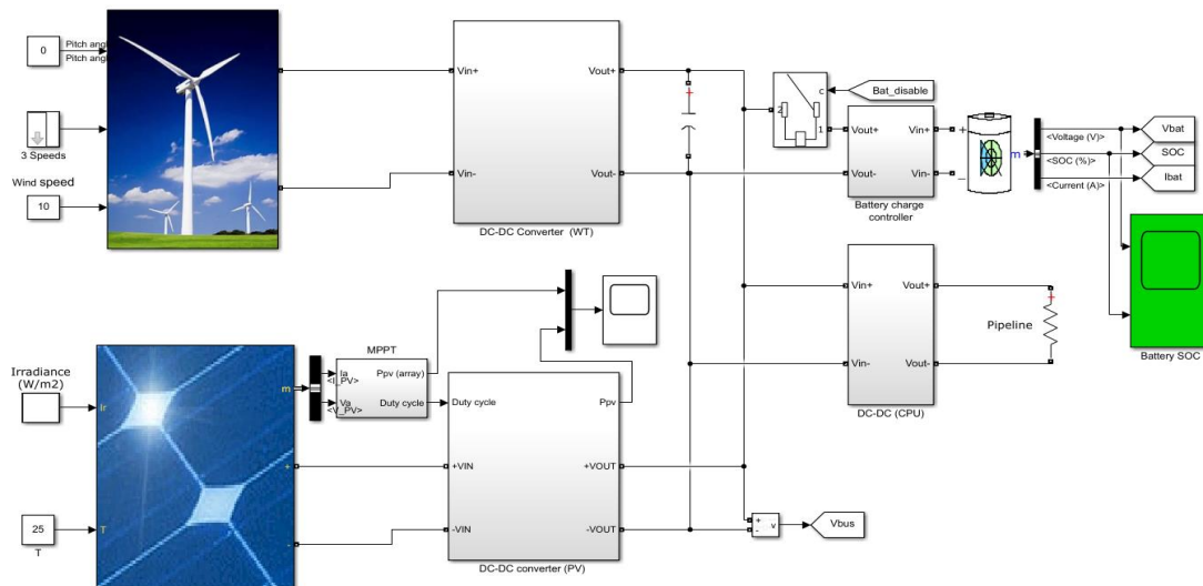
Fig. 2. Simulink model of an off-grid WT-PV hybrid system.
