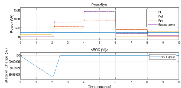
Fig. 11. Power flow and Battery State of Charge (SOC).
