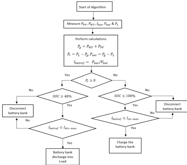
Fig. 5. Flow chart of the battery control algorithm.
