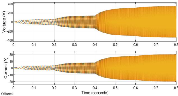
Fig. 9. Generated voltage and load current for different wind speeds.
